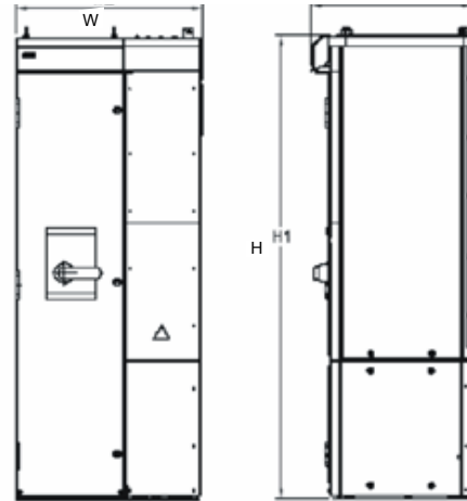
Floor Mount (UX1-7 - UX1-8)
